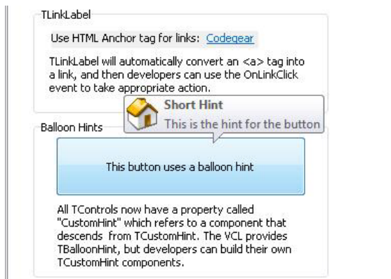
Figure 16 Balloon Hints
