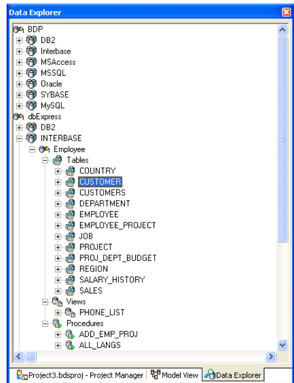
Figure 9 Data Explorer
