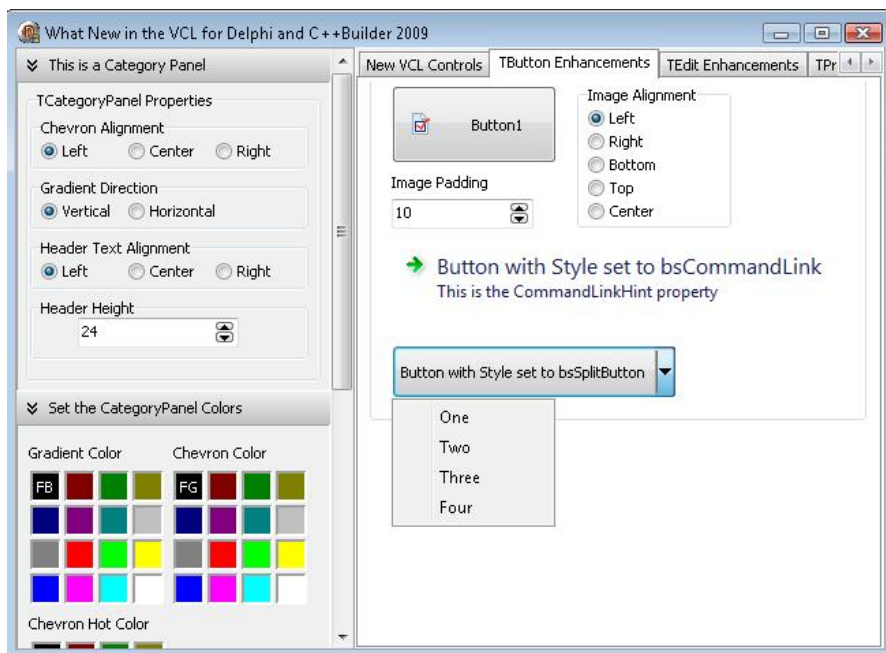
Figure 17 Panel Group
