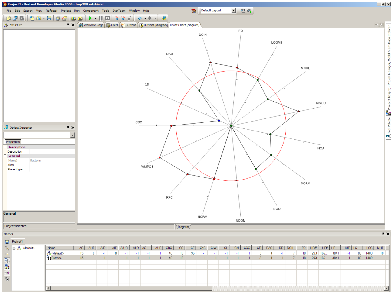
Figure 34 Metrics Analysis
