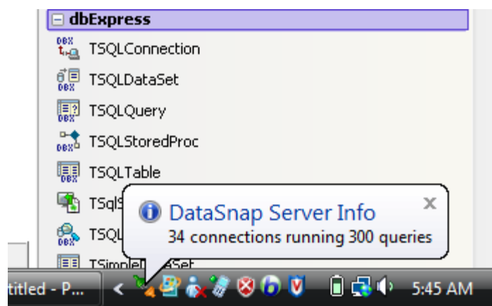
Figure 21 Tray Icon
