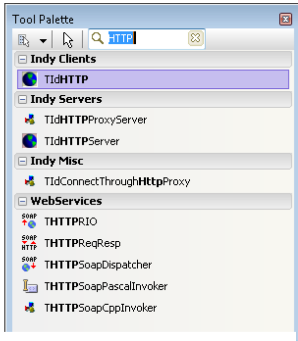
Figure 5 Component Search
