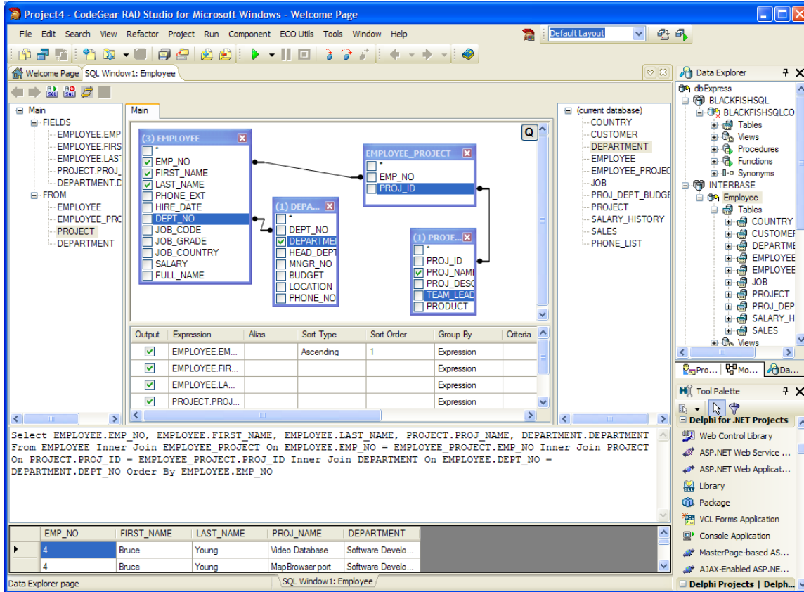
Figure 10 SQL Window
