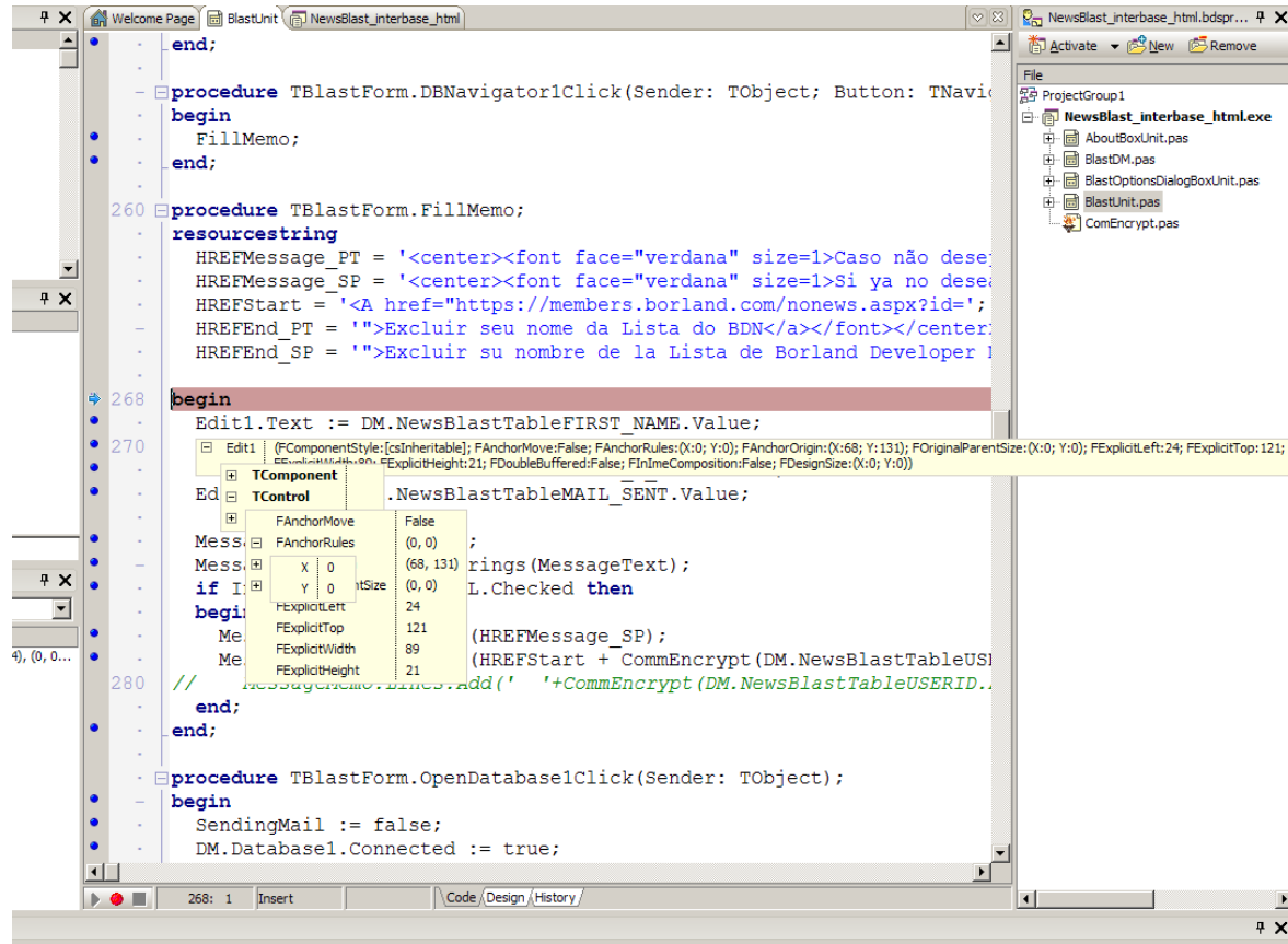
Figure 11 Debugger
