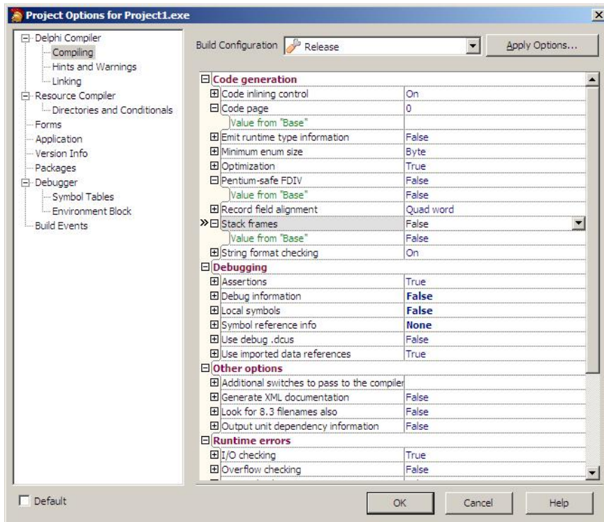
Figure 1 Build Configurations
