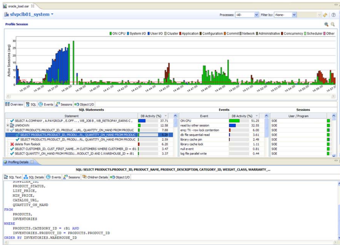
Figure 4: Predicate Analysis
